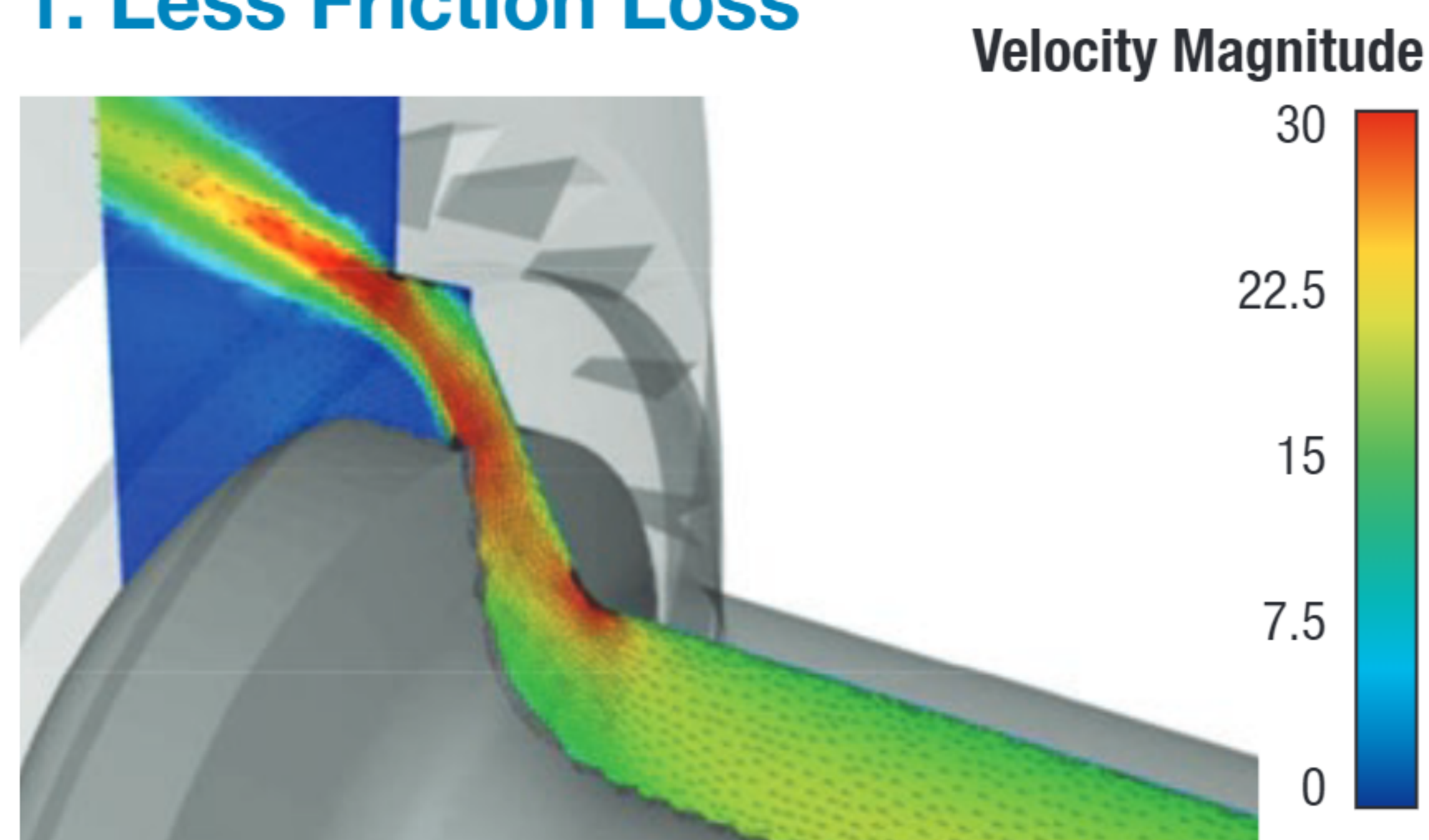
Image 1a: Velocity of Water – Spinning teeth
