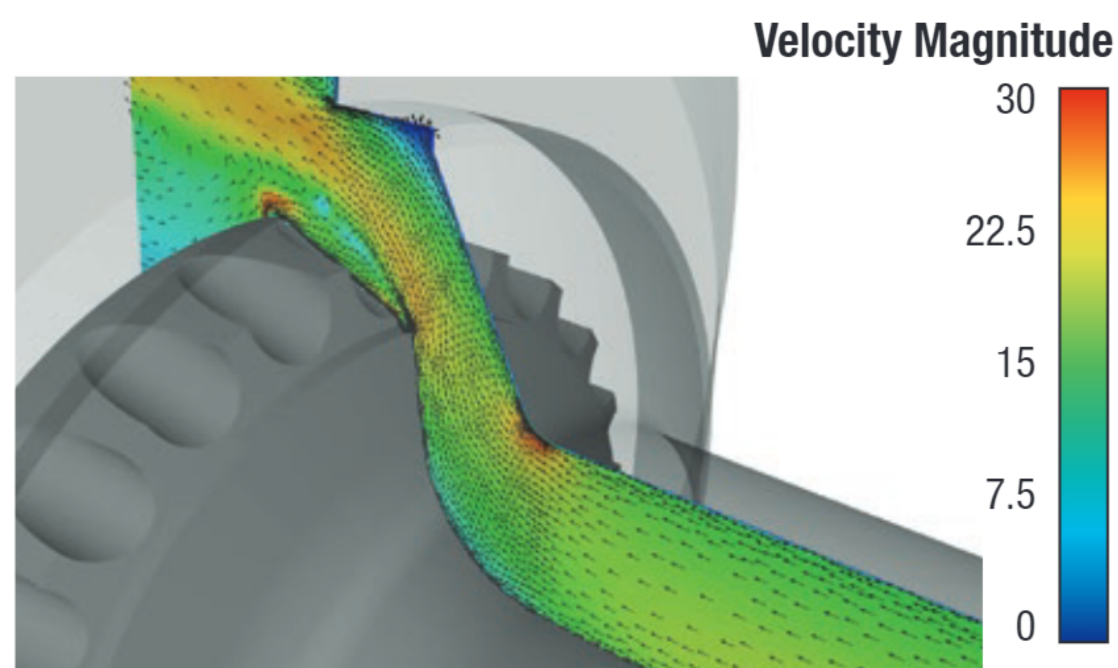
Image 1b: Velocity of Water – RYLSTATIC®
