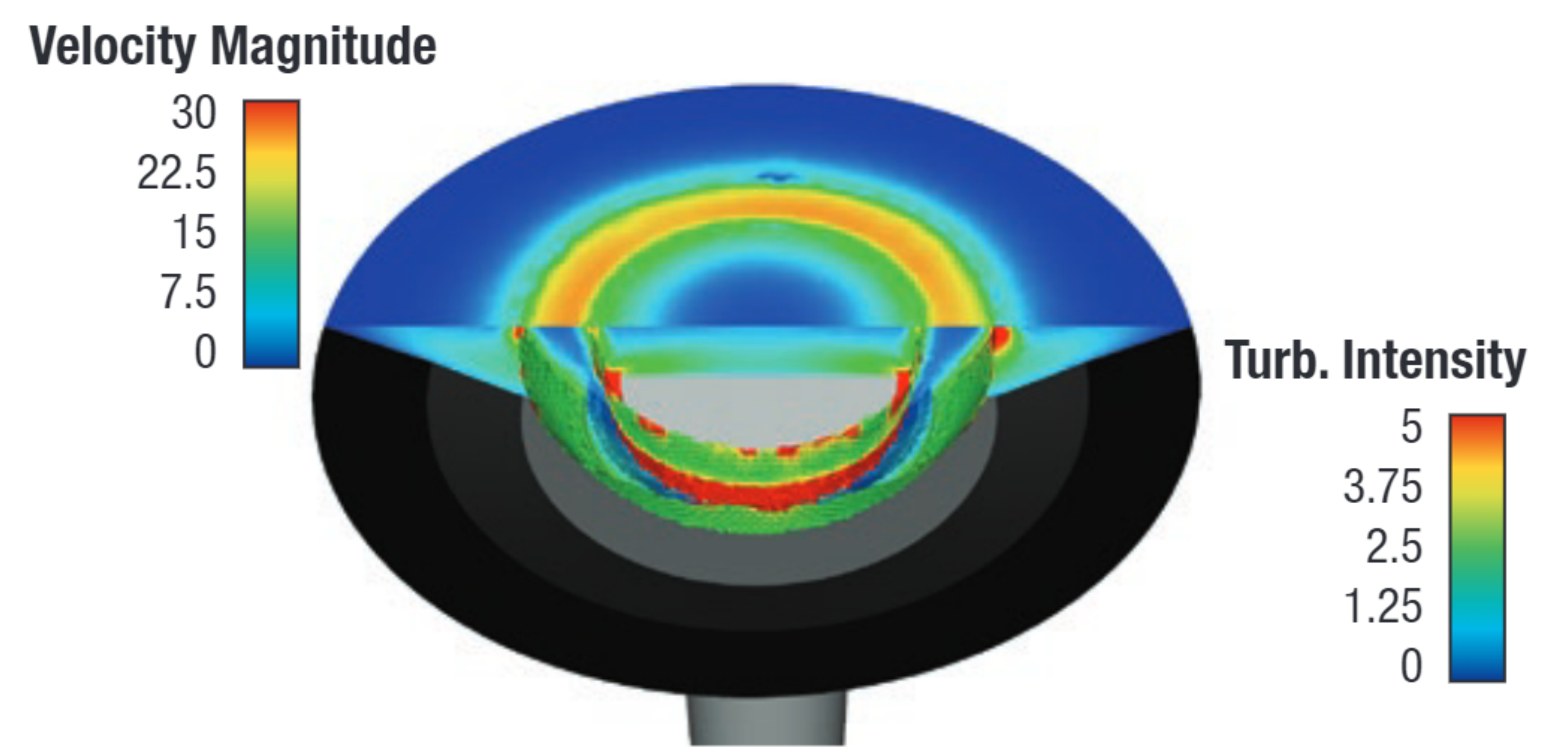
Image 6: Speed Magnitude vs Turbulence Intensity (RYLSTATIC®)
