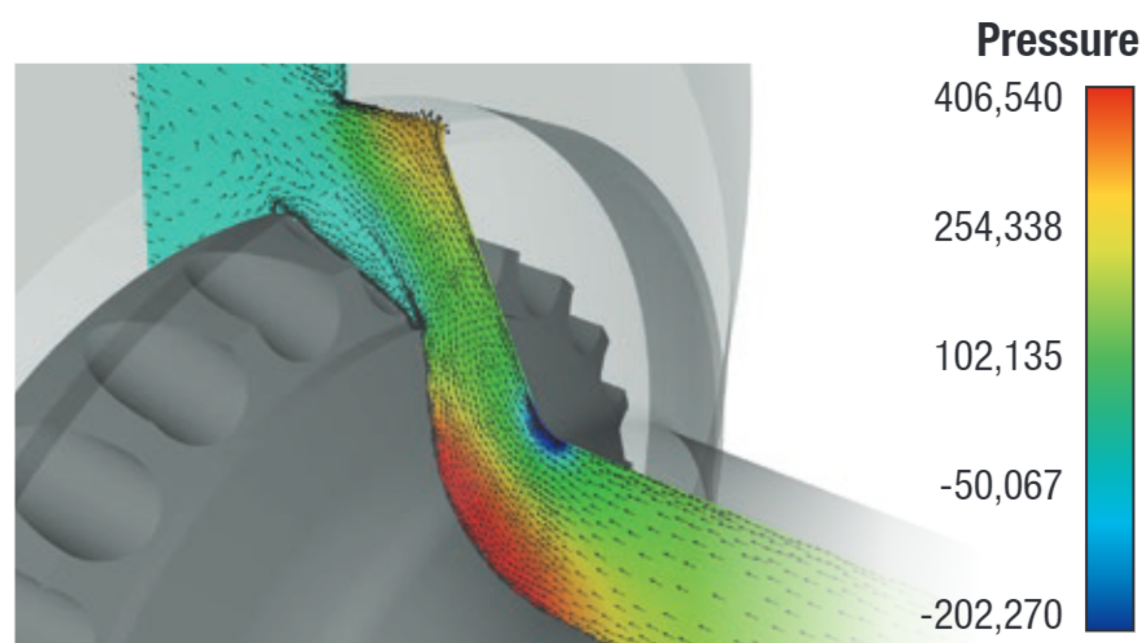
Image 2b: Static Pressure Distribution – RYLSTATIC®
