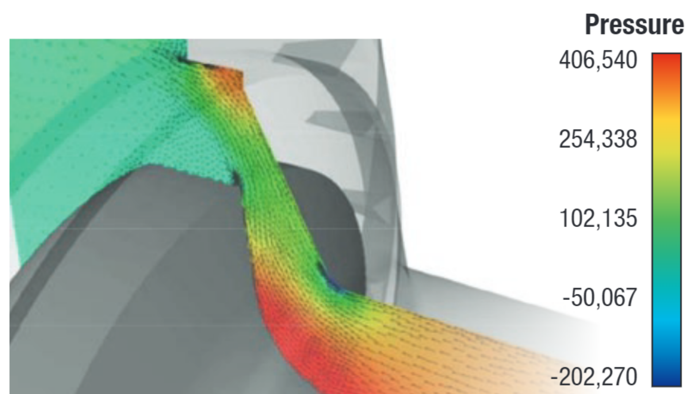
Image 2a: Static Pressure Distribution – Spinning Teeth
